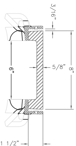
R-4990-AX TYPICAL SECTION TYPE "P" GRATE W/ TYPE "B" FRAME (SCALE: 1/4"=1")
