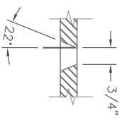
VENT HOLE DETAIL SCALE 1: 4
