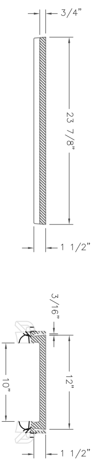
R-4990-CX TYPE "E" LID WITH TYPE "B" FRAME TYPICAL SECTION
