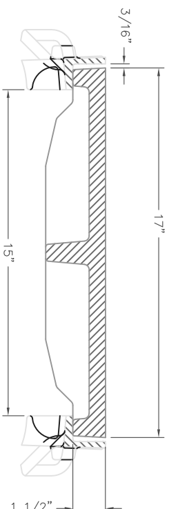
R-4990-EX TYPE "E" VENTED LID WITH TYPE "B" FRAME TYPICAL SECTION (SCALE: 1/4"=1")
