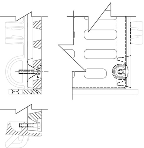
FRAME & GRATE SHOWING DEBRIS CHUTE SCALE 1:4
