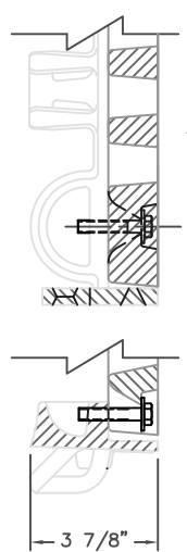
FRAME & GRATE SHOWING DEBRIS CHUTE SCALE 1:4
