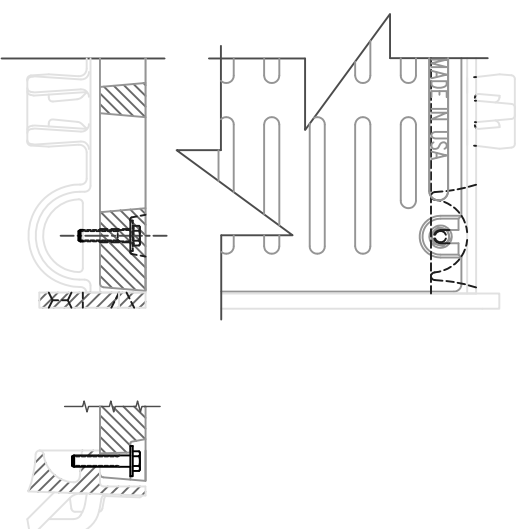
FRAME & COVER SHOWING DEBRIS CHUTE
