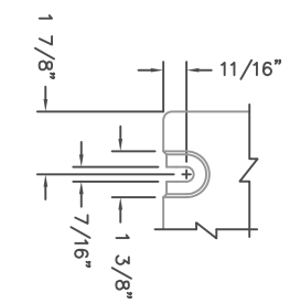
BOLT SLOT DETAIL SCALE 1:4
