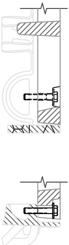
FRAME & GRATE SHOWING DEBRIS CHUTE SCALE 1:4
