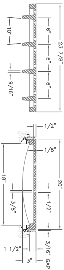
R-4999-FX RIVERWALK TYPE "K" GRATE WITH TYPE "B" FRAME TYPICAL SECTION
