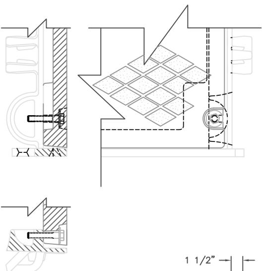
FRAME & COVER SHOWING DEBRIS CHUTE SCALE 1:4
